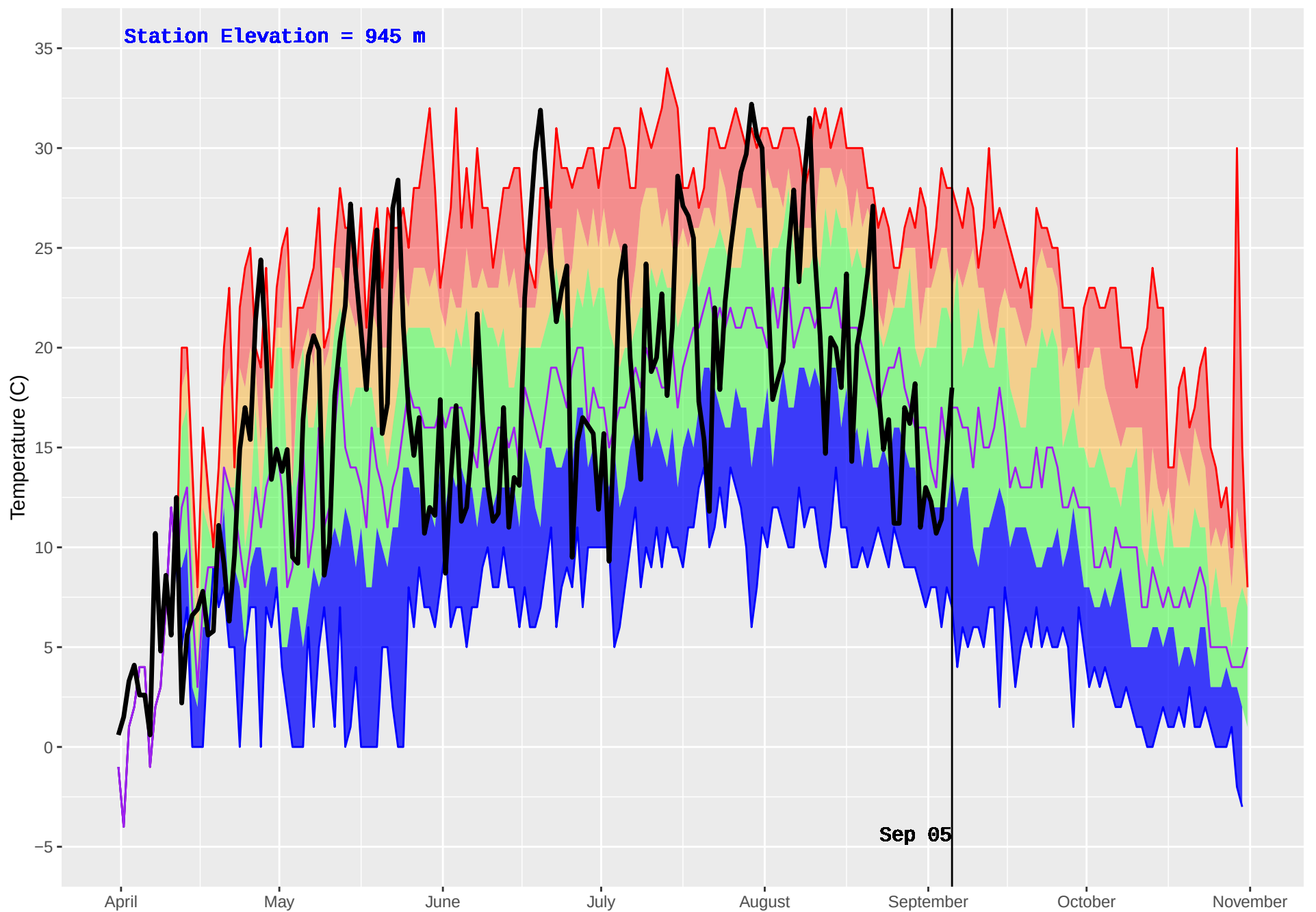
BOWRON HAGGEN (193) : Historical (1986–2016) and Current (2018) Daily Temperature
