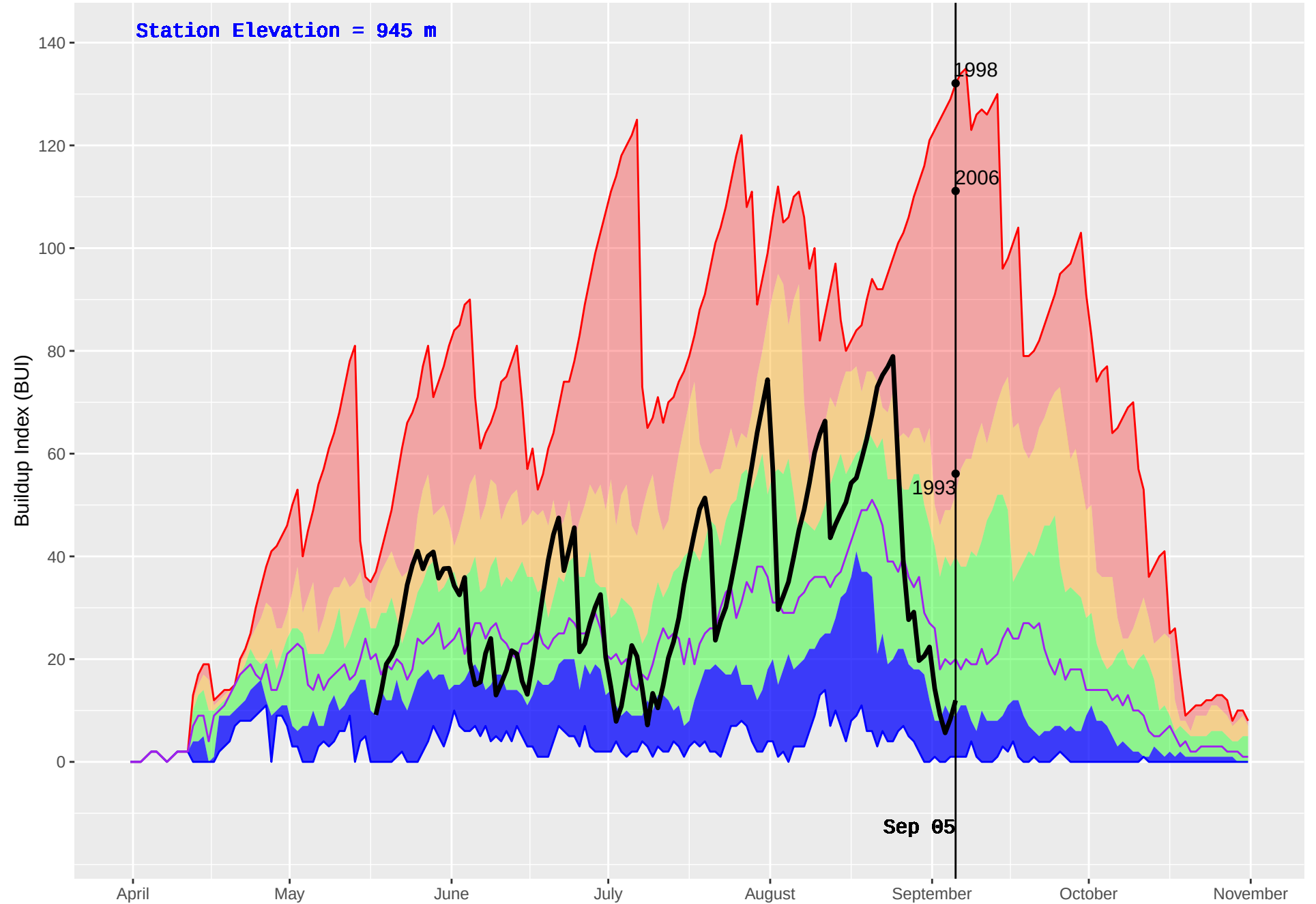
BOWRON HAGGEN (193) : Historical (1986–2016) and Current (2018) Daily Buildup Index (BUI)
